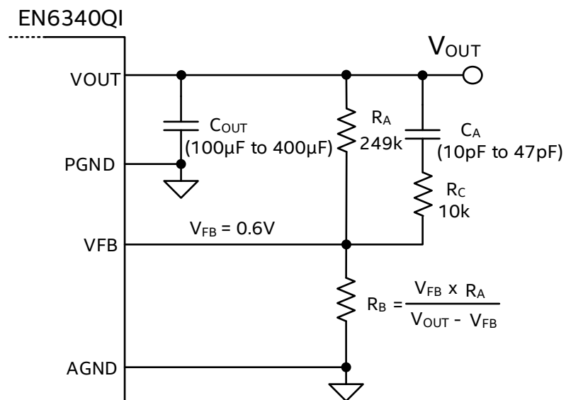
Figure 5: V_{OUT} Resistor Divider & Compensation Capacitor
